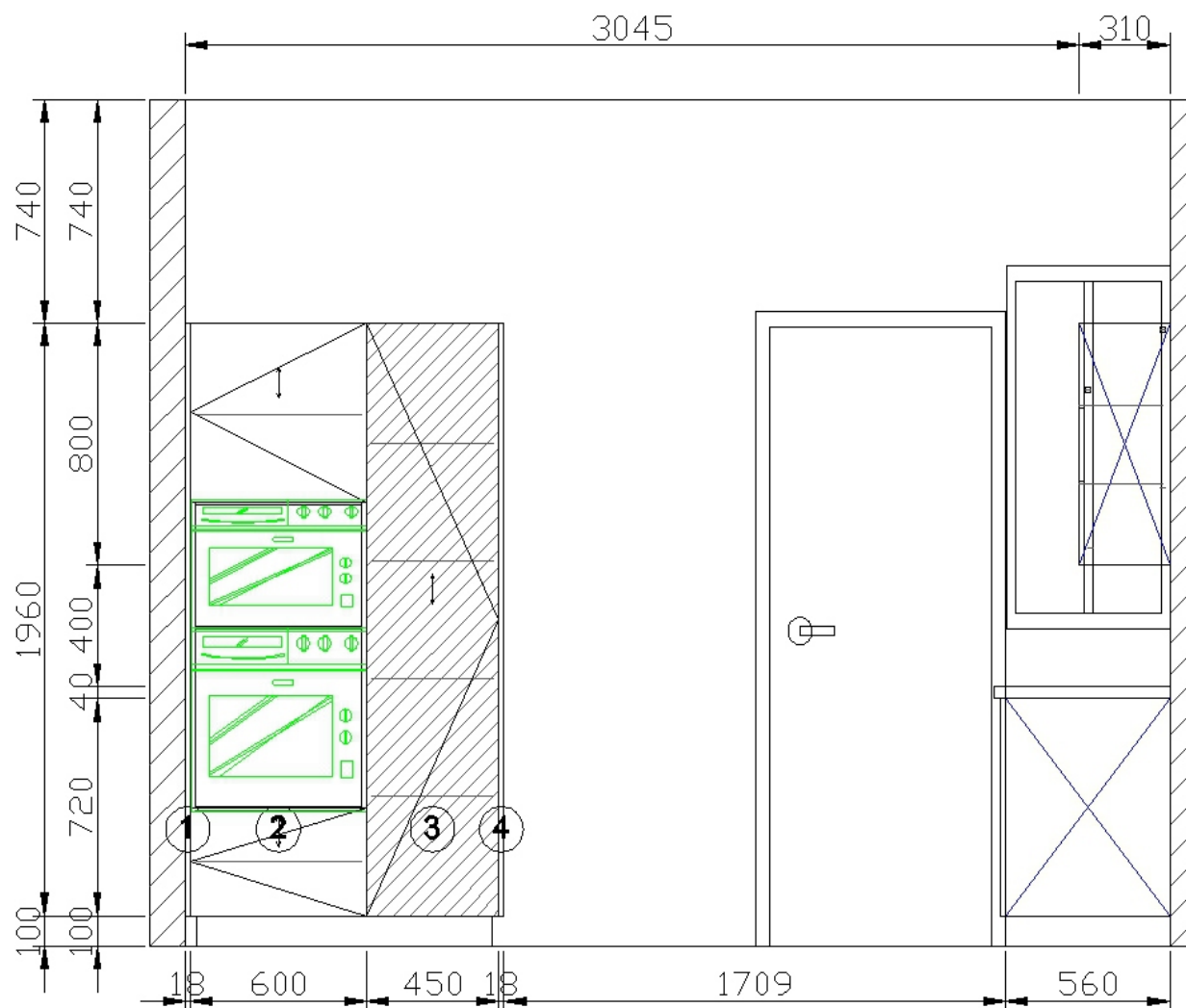
A View elevation drawing
