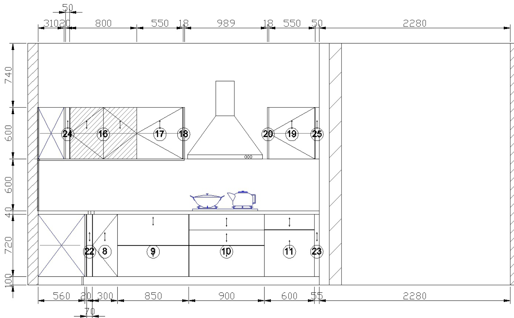
C View elevation drawing
